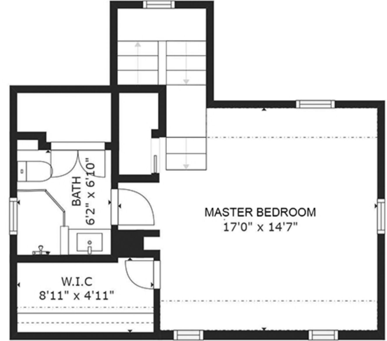
FLOOR 3
