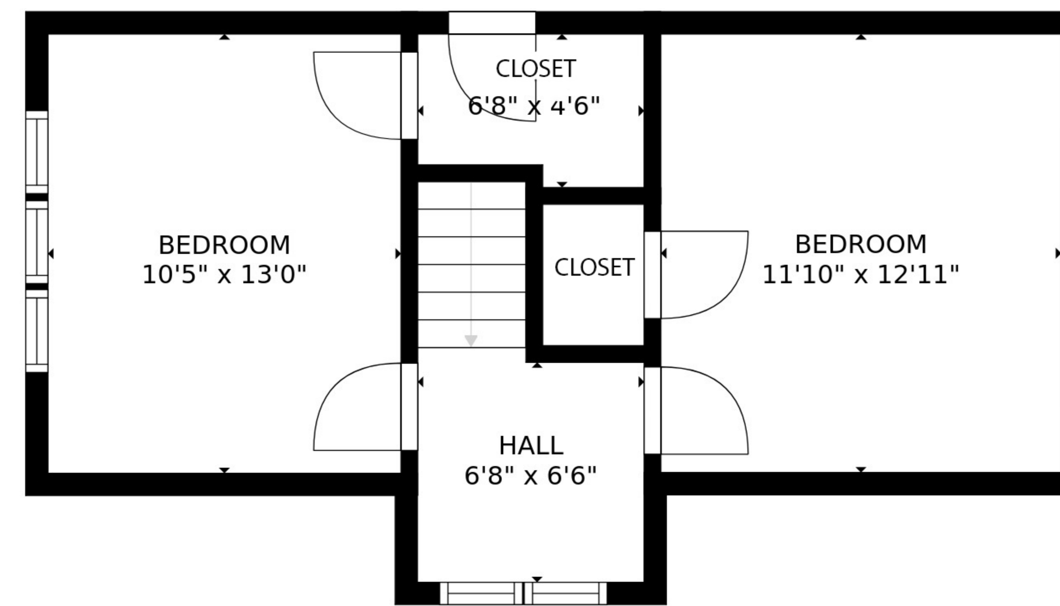
UPPER LEVEL
